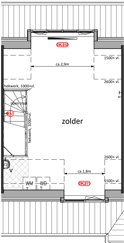
Tweede Verdieping DK.211 = Dakkapel ca.1,8m DK.212 = Dakkapel ca.2,9m
