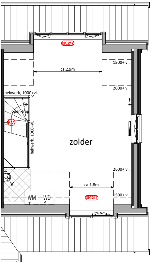
Tweede Verdieping DK.211 = Dakkapel ca.1,8m DK.212 = Dakkapel ca.2,9m
