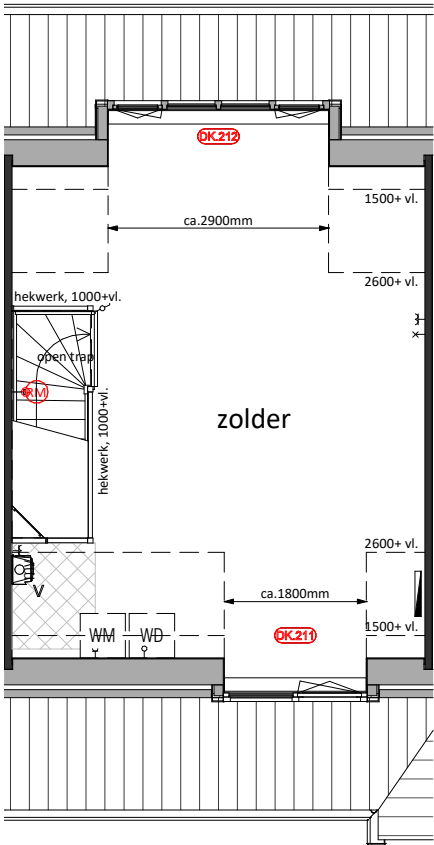
Tweede Verdieping DK.211 = Dakkapel ca.1800mm DK.212 = Dakkapel ca.2900mm
