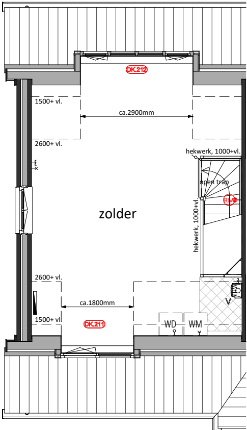
Tweede Verdieping DK.211 = Dakkapel ca.1800mm DK.212 = Dakkapel ca.2900mm
