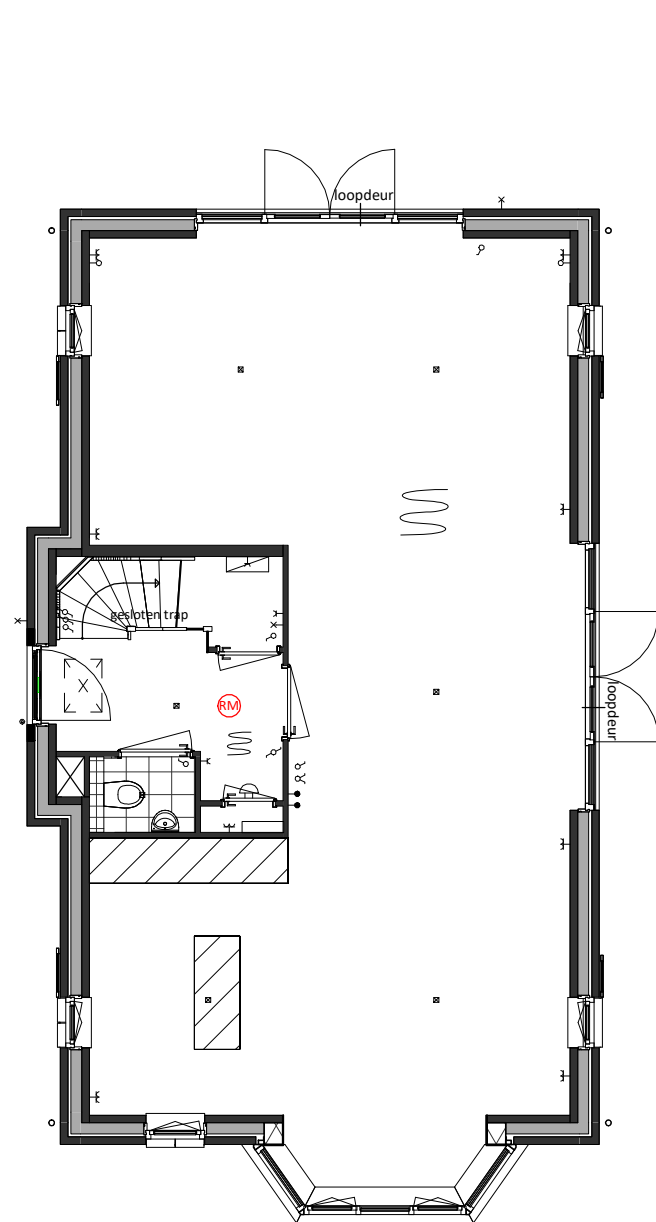
Begane grond Basis
