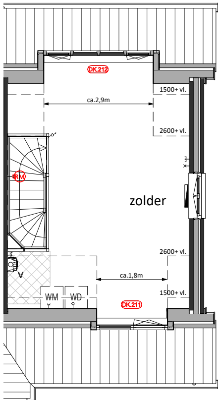
Tweede Verdieping DK.211 = Dakkapel ca.1,8m DK.212 = Dakkapel ca.2,9m
