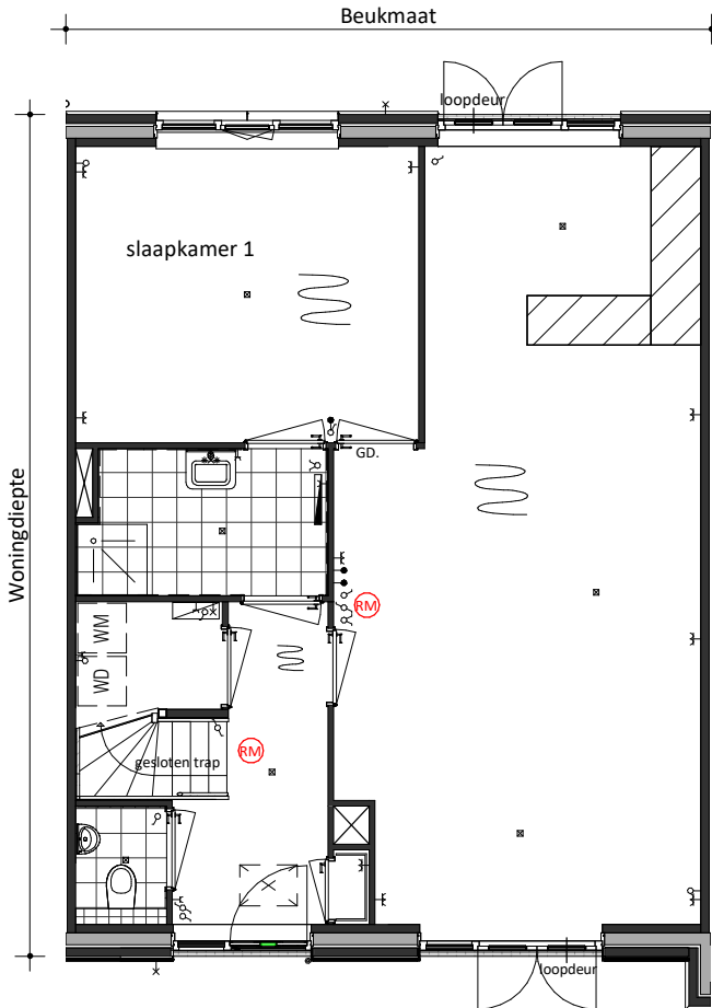
Begane Grond Basis
