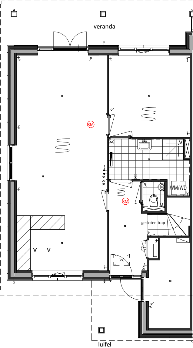
Begane Grond Basis
