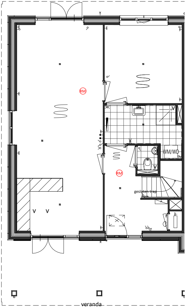
Begane Grond Basis
