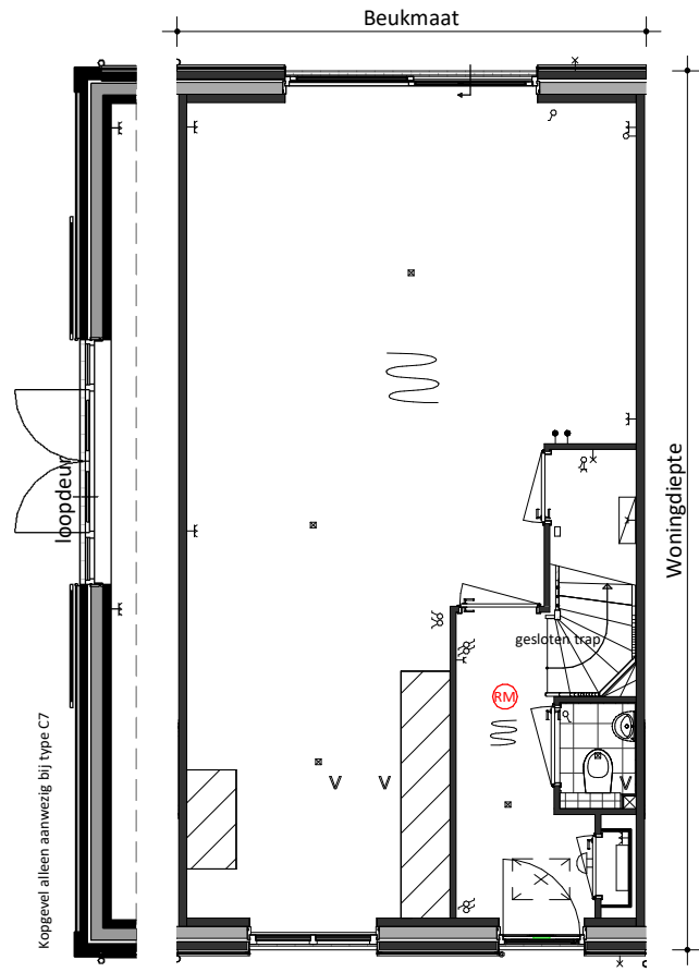
Begane grond Basis
