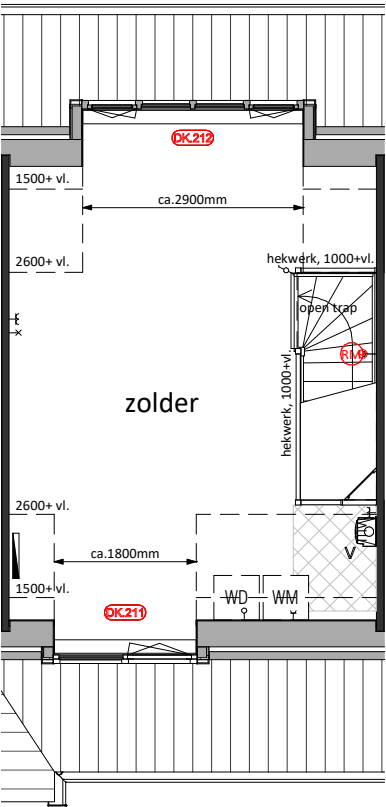
Tweede Verdieping DK.211 = Dakkapel ca.1800mm DK.212 = Dakkapel ca.2900mm
