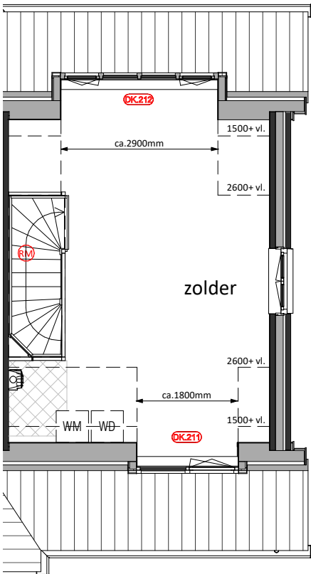
Tweede Verdieping DK.211 = Dakkapel ca.1800mm DK.212 = Dakkapel ca.2900mm
