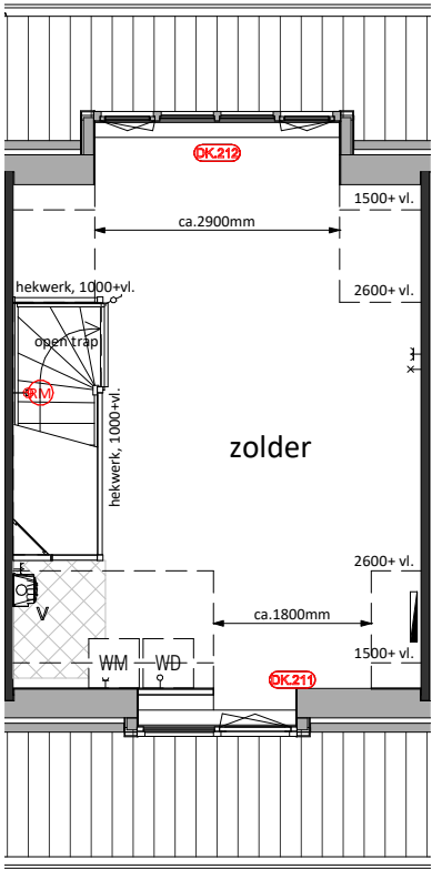
Tweede Verdieping DK.211 = Dakkapel ca.1800mm DK.212 = Dakkapel ca.2900mm
