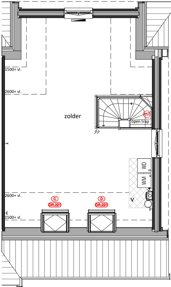
Tweede verdieping DR.221 = Extra houten tuimeldakraam (ca.980 x 940mm)
