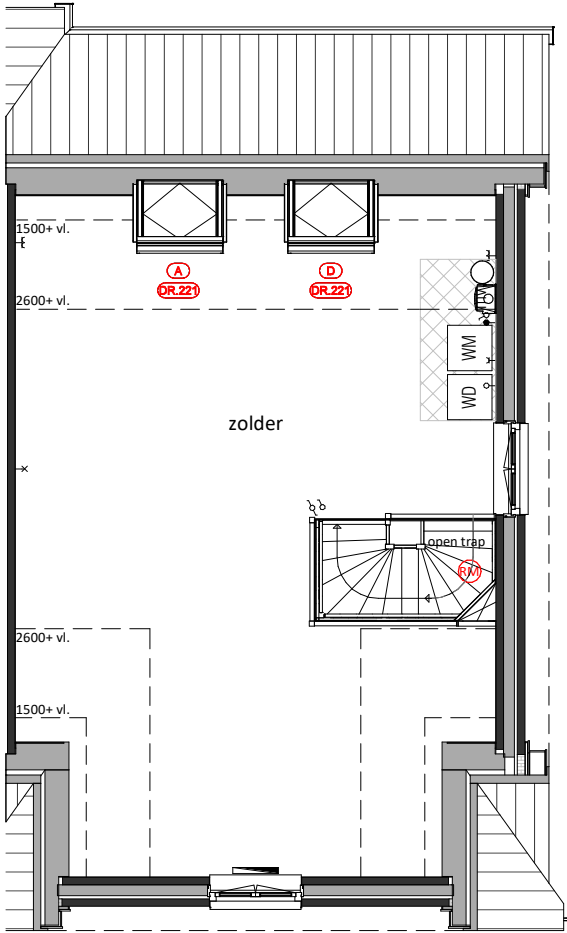
Tweede verdieping DK.221 = Dakraam (ca.980 x 940mm)
